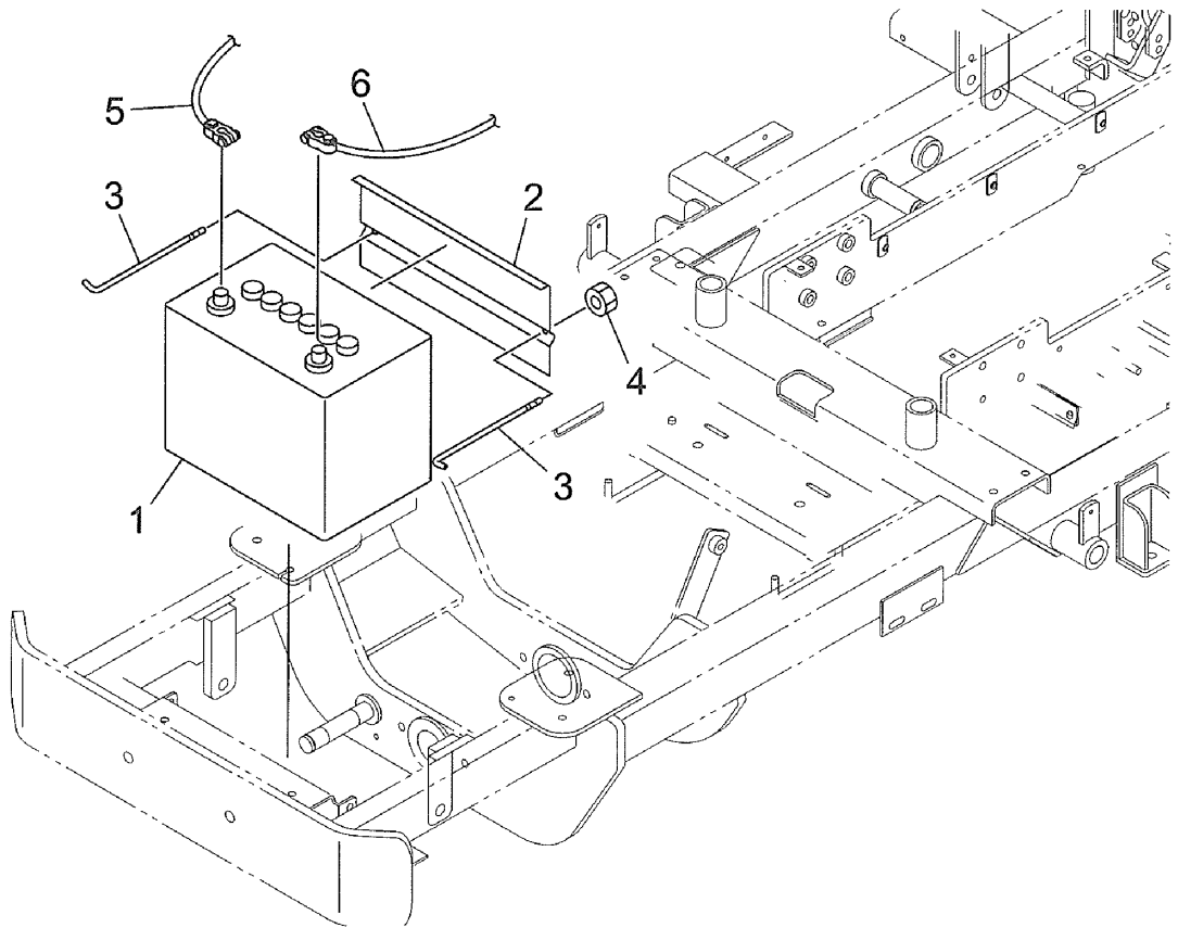
BATTERY
