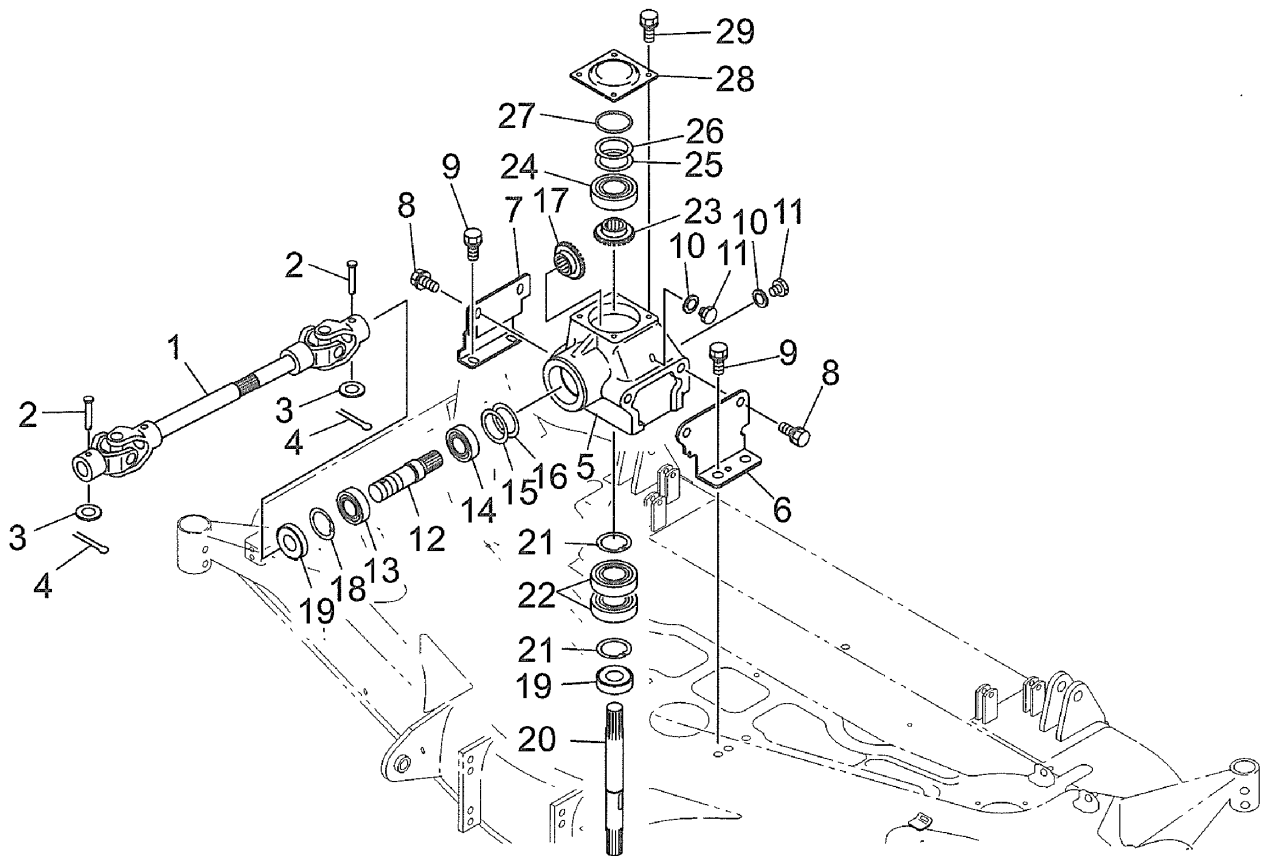
FIG.304 クドウ DRIVING
